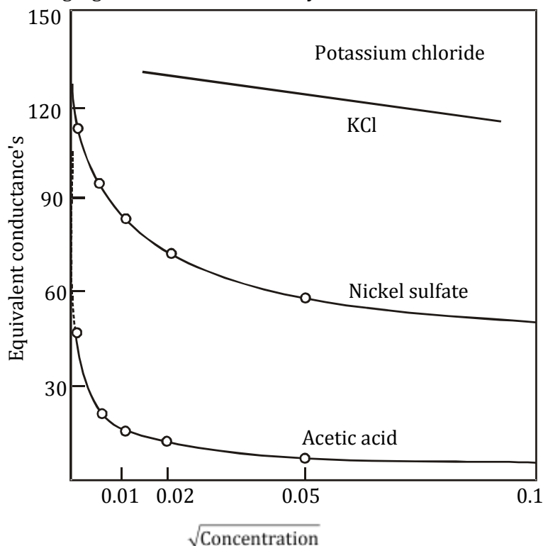
Conductance of electrolytes of different types
